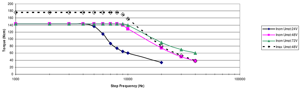
Motor: sm268ht-KF4.2A-008 Drive:smd276 Umotor: 24V, 48V, 72V Inom: 4.2A Imax:7A 1000 Steps/Rev
