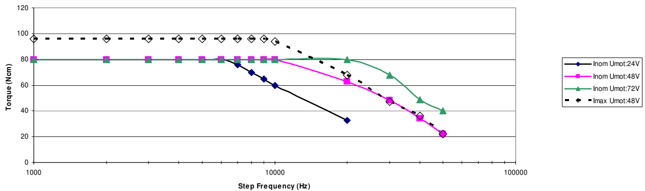
Motor: sm267ht-KF4.2A-008 Drive:smd276 Umotor: 24V, 48V, 72V Inom:4.2A Imax:6A 1000 Steps/Rev
