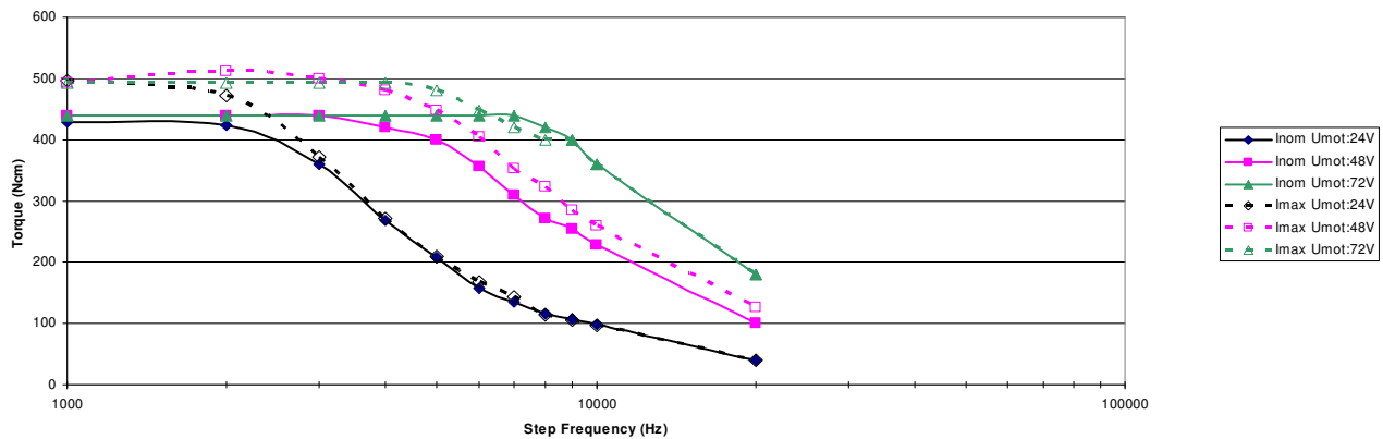
Motor: sm2913ht-KF7.0A-008 Drive:smd276 Umotor: 24V, 48V, 72V Inom: 7.0A Imax:8A 1000 Steps/Rev
