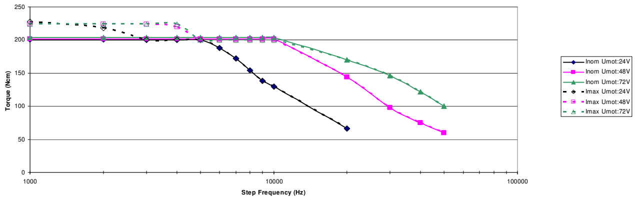
Motor: sm299ht-KF7.0A-008 Drive:smd276 Umotor: 24V, 48V, 72V Inom: 7.0A Imax:8A 1000 Steps/Rev
