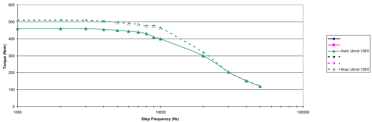
Motor: sm2913ht-KF7.0A-008 Drive:smd285 Umotor: 130V Inom: 7.0A Imax:8A 1000 Steps/Rev
