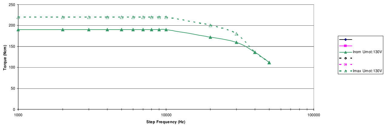
Motor: sm299ht-KF7.0A-008 Drive:smd285 Umotor: 130V Inom: 7.0A Imax:8A 1000 Steps/Rev
