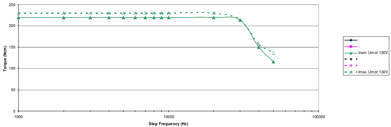
Motor: sm299ht-KF7.0A-008 Drive:smd298 Umotor: 130V Inom: 7.0A Imax:8A 1000 Steps/Rev
