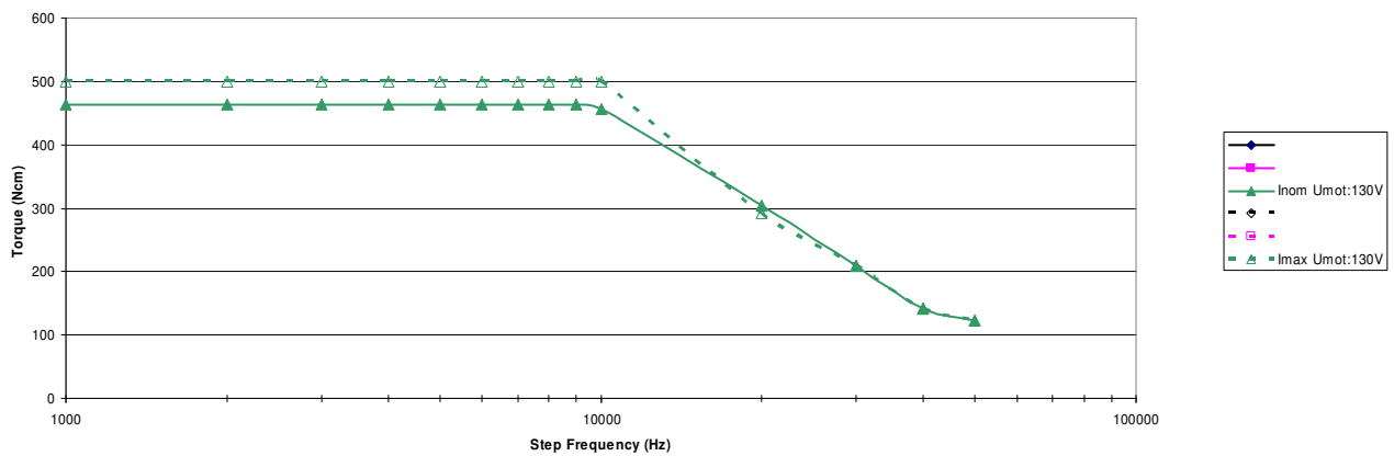
Motor: sm2913ht-KF7.0A-008 Drive:smd298 Umotor: 130V Inom: 7.0A Imax:8A 1000 Steps/Rev
